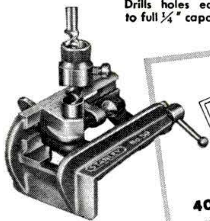
No. 59 Doweling Jig For boring holes accurately and easily in the edge, end or surface of boards. Furnished with depth gauge and six guides — \frac{3}{16} , \frac{1}{4} , \frac{5}{16} , \frac{3}{8} , \frac{7}{16} , \frac{1}{2} ".
